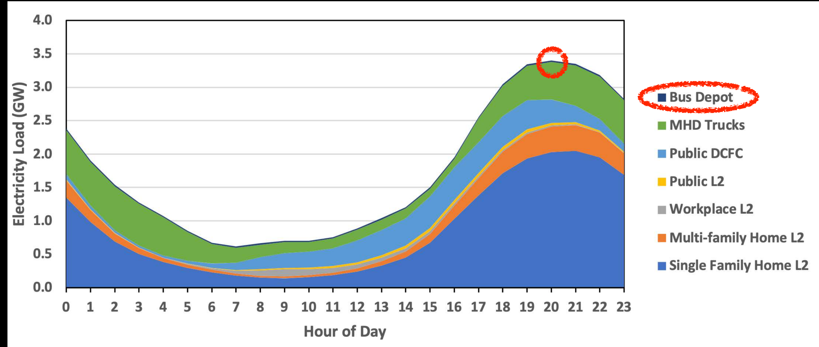
Statewide EV Load Shape for Strong Electrification Policy Scenario
