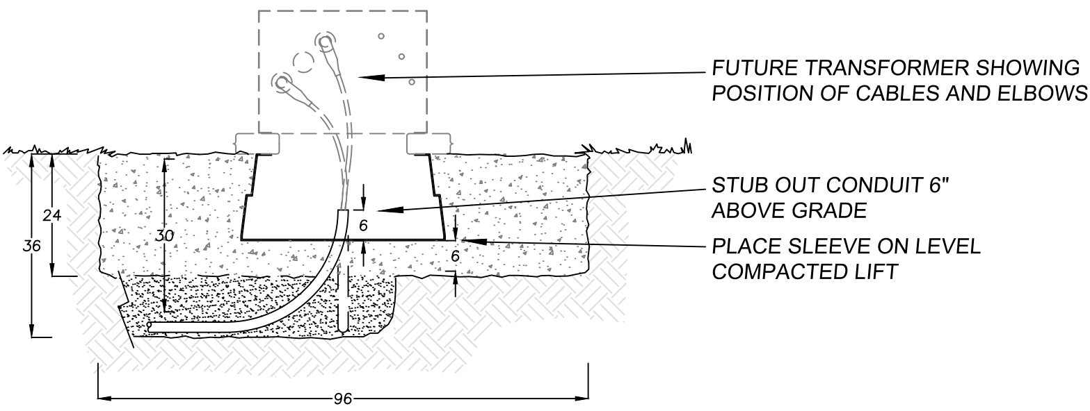
PROFILE - CONDUIT & EQUIPMENT SLEEVE
